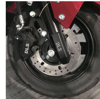
Front Disc
